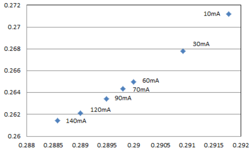
(3) Forward Current vs. Chromaticity Coordinate (Temp: 25°C)
