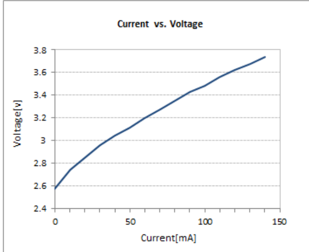
(1) Forward Voltage vs Forward Current
