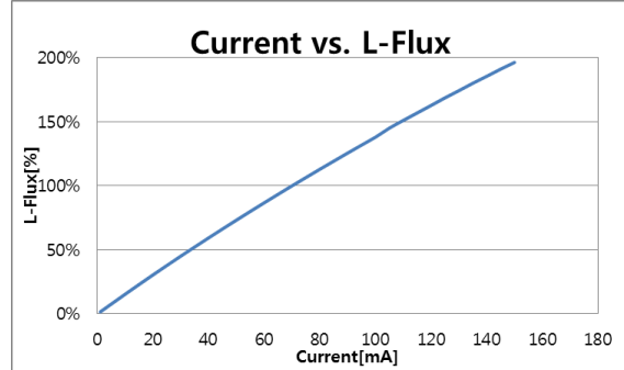
(2) Relative Luminosity vs. Forward Current
