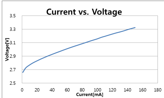
(1) Forward Voltage vs. Forward Current
