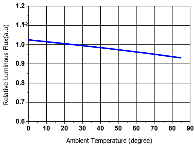
(5) Relative Luminous Flux vs Ambient Temperature
